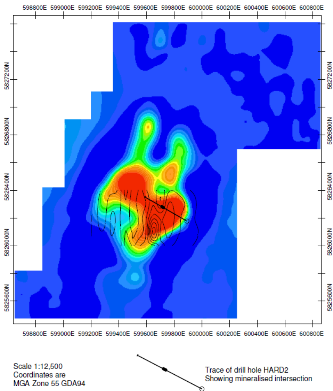
Figure 2: Three Mile Prospect – 3D magnetic model at RL 0m Contours are of fixed loop X component at 0.48ms
